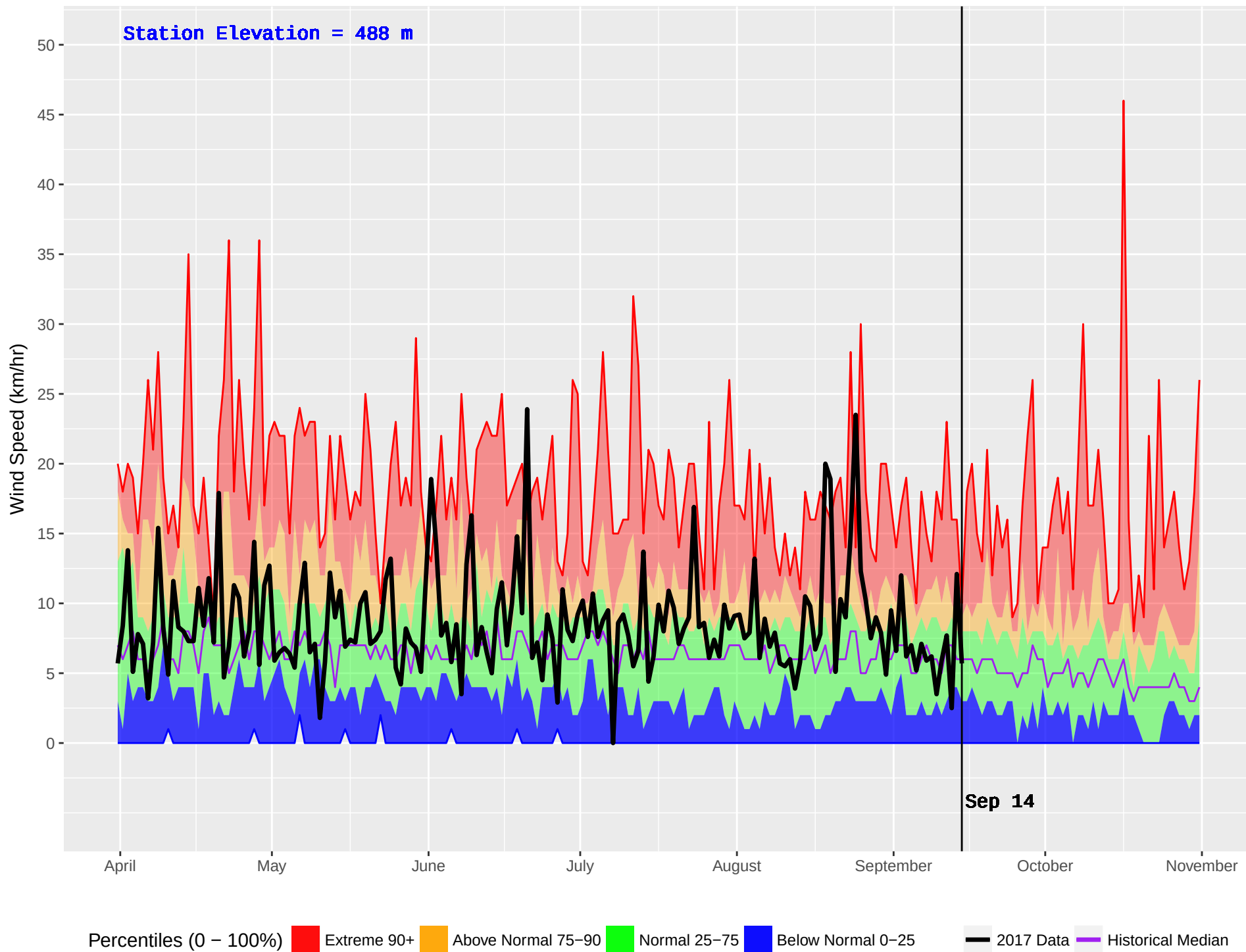
MABEL LAKE 2 (362) : Historical (1987–2016) and Current (2017) Noon Wind Speed
