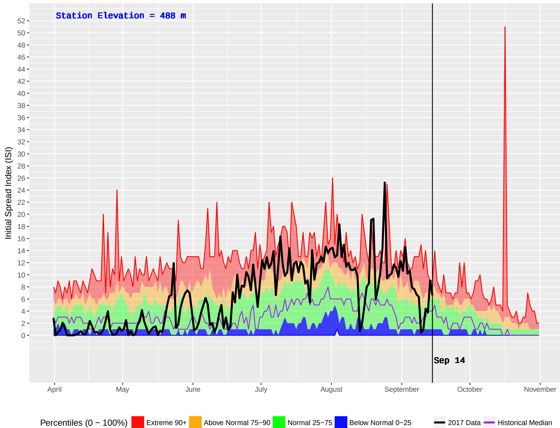
MABEL LAKE 2 (362) : Historical (1987–2016) and Current (2017) Noon Initial Spread Index (ISI)
