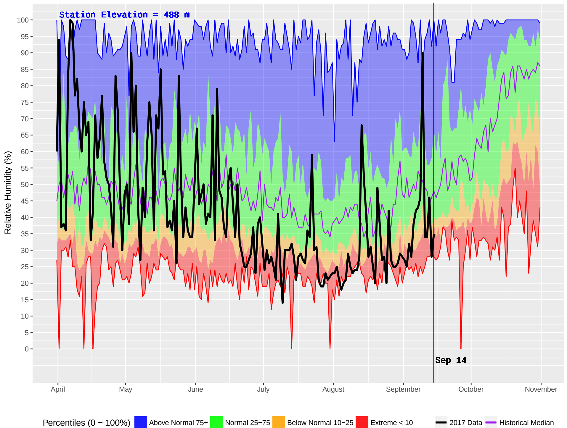
MABEL LAKE 2 (362) : Historical (1987–2016) and Current (2017) Noon Relative Humidity
