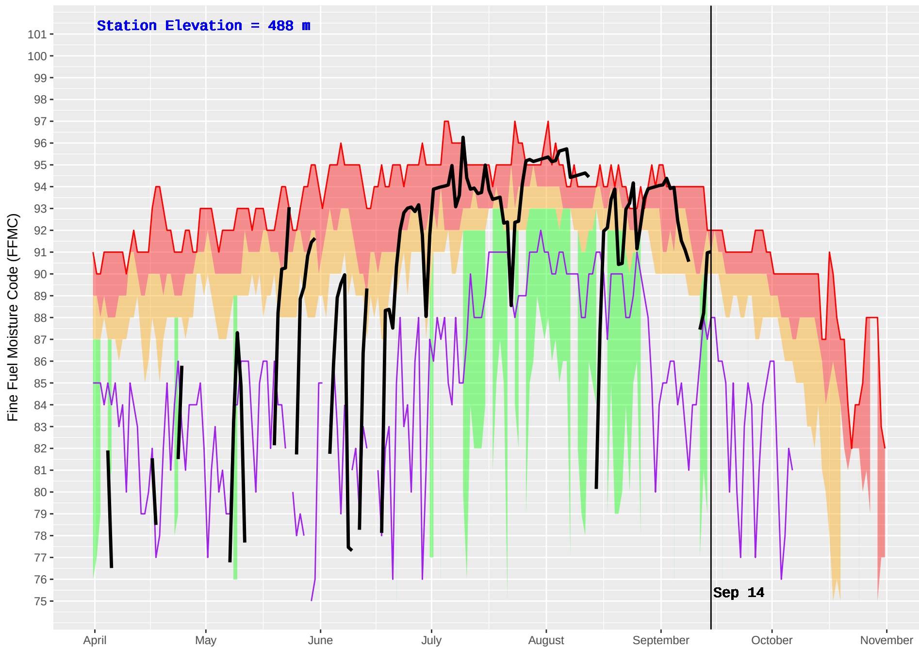
MABEL LAKE 2 (362) : Historical (1987–2016) and Current (2017) Noon Fine Fuel Moisture Code (FFMC)
