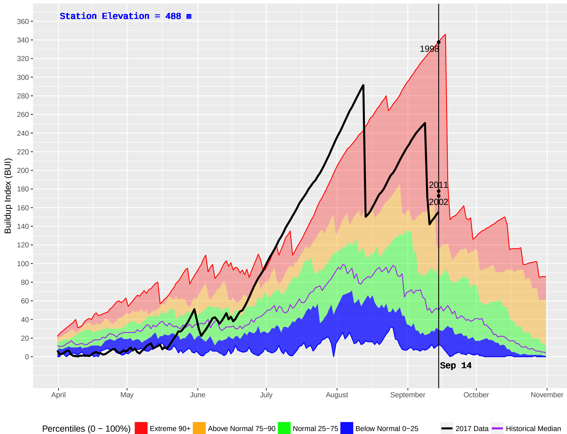
MABEL LAKE 2 (362) : Historical (1987–2016) and Current (2017) Noon Buildup Index (BUI)
