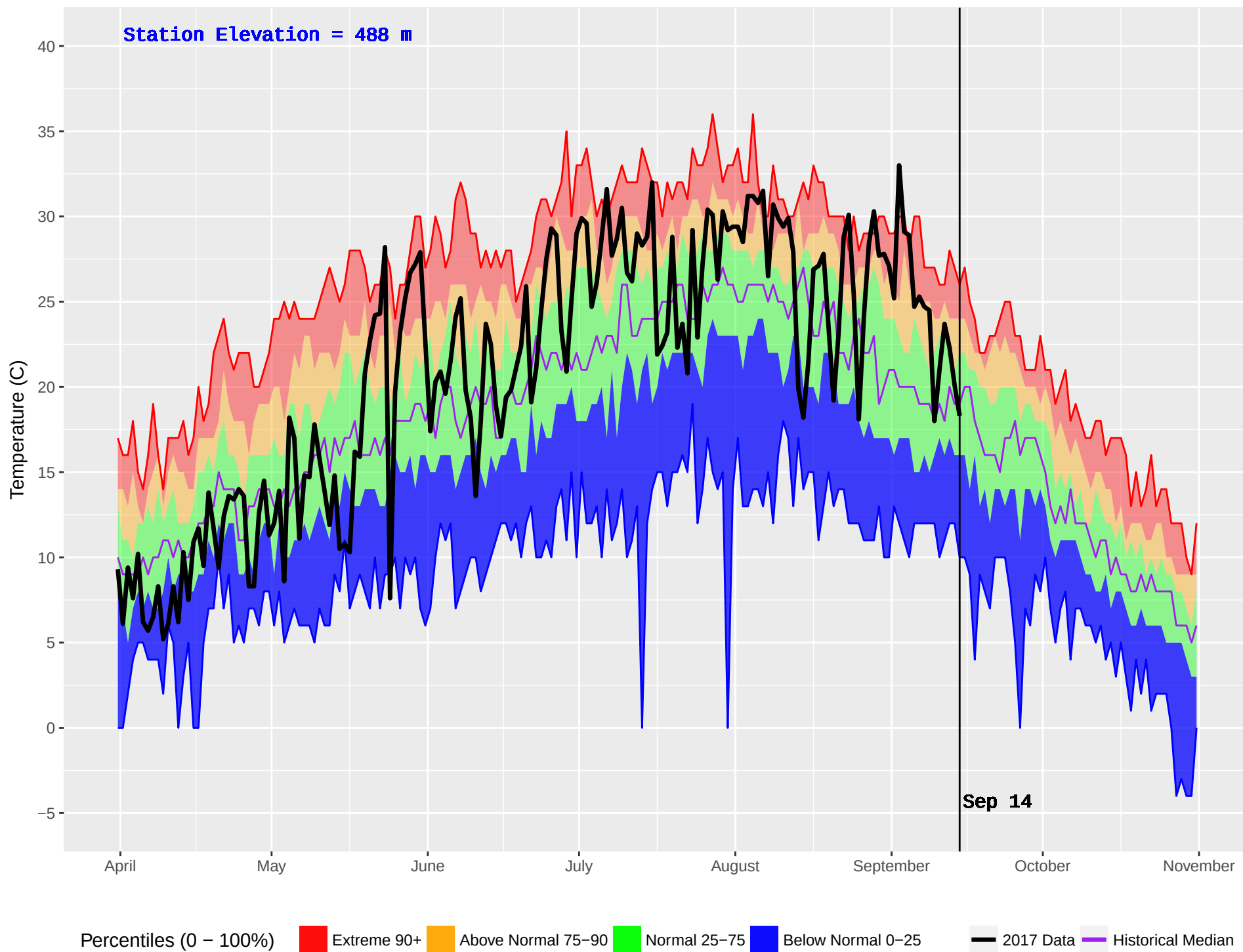
MABEL LAKE 2 (362) : Historical (1987–2016) and Current (2017) Noon Temperature
